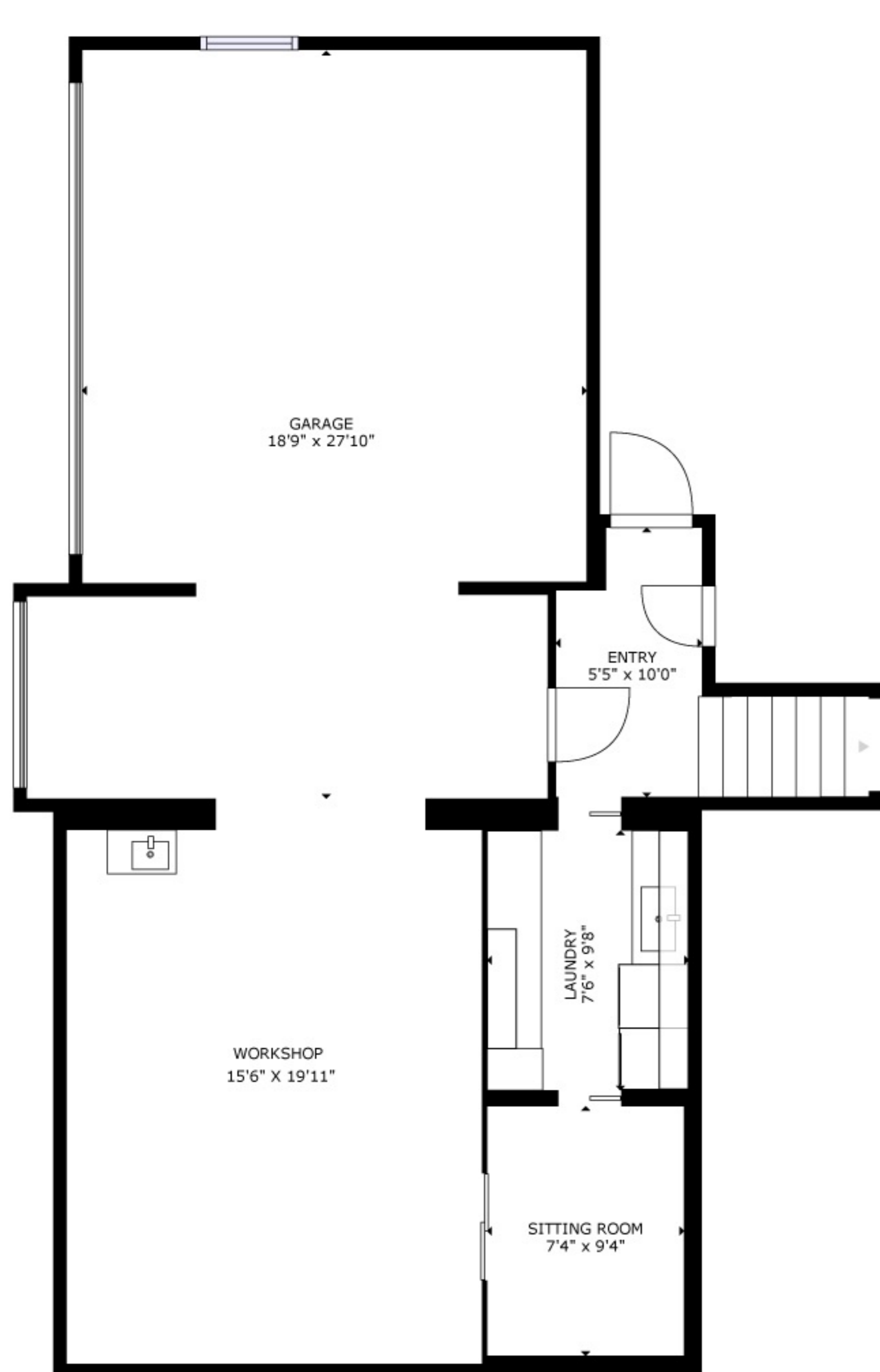
FLOOR 1
